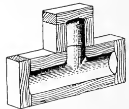
FIG. 571. CORE-BOX FOR TEE-PIPE FITTING.
